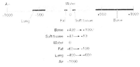
Fig. 1.4 The Hounsfield scale of CT numbers
